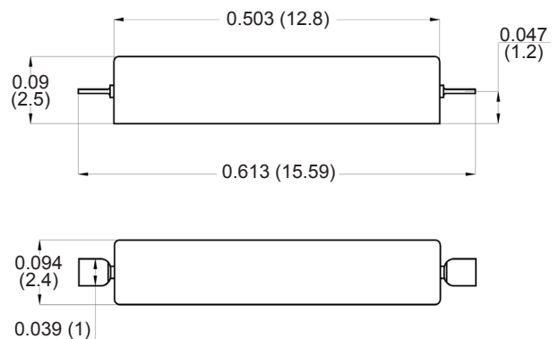
RI-60-81 Axial
