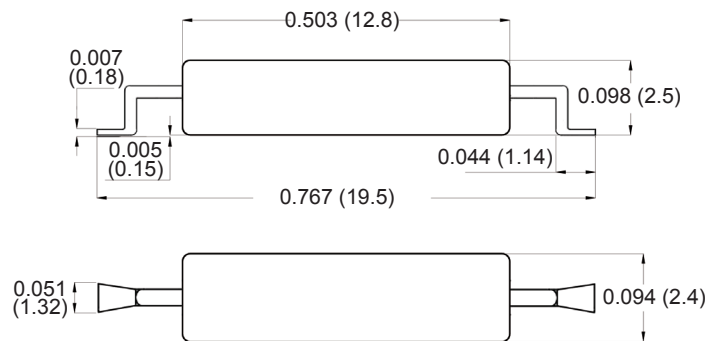
RI-60-91 SMD
