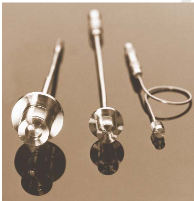
From left to right, KD-1975, KD-1950 and KD-1925 high temperature displacement sensors
