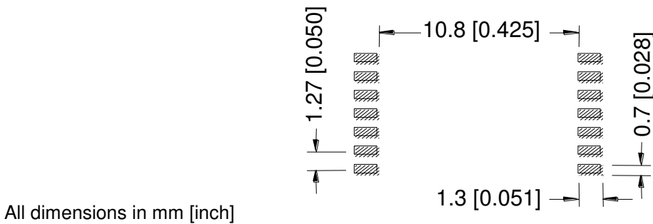
Fig. 9: Recommended pad-layout for MS5536-CPJU / MS5536-CNJU
