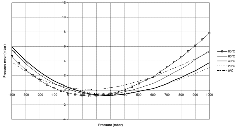
Absolute Pressure Accuracy after Calibration for MS5536-CPJU
