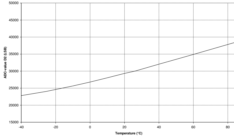
ADC-value D2 vs Temperature (typical)
